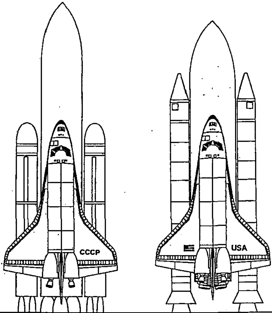
Soviet Reusable Space System
